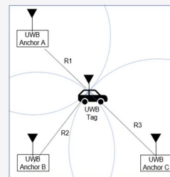
기존 · 3-Anchor Triangulation
